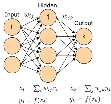
Fig. 1. Architecture of an MLP. Each layer is fully connected to the previous and following layer whereas within each layer the neurons are not connected. The index i is labeling the input features x and indices j, k are labeling the neurons in each layer, where x are the input features, w are the weights and z are the weighted sums of inputs and y activations.
