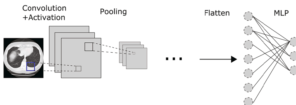
Fig. 2. Typical architecture of a CNN. In the first stage feature extraction is performed using convolutional and pooling layers, typically there are several such layers connected to each other which makes the network “deep”. The second stage consists of a MLP which is using the extracted features to perform class predictions.
